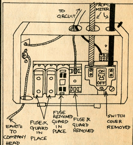
Consumer Box
